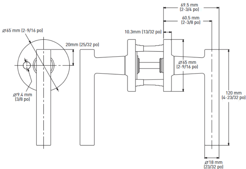
LOQUET 6-EN-1 VERROUILLABLE/NON VERROUILLABLE
